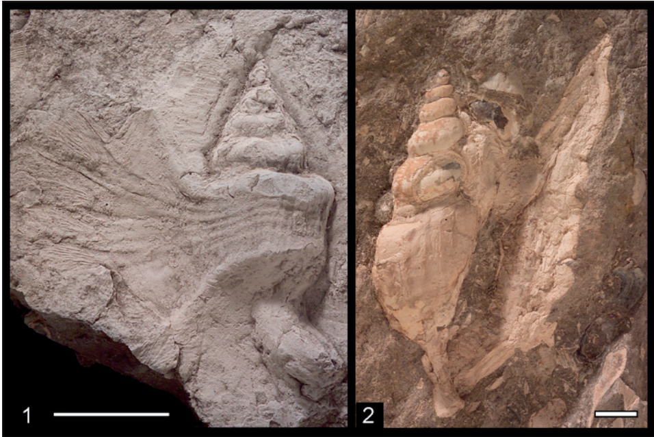
Fig. 6. 6.1 Harpodactylus pinnipenna (ZEKELI, 1852), Holotype, Blahberg (Windischgarsten, Upper Austria), Geologische Bundesanstalt Vienna. Specimen coated with natrium chloride ; 6.2. Rhombovermeria passer (ZEKELI, 1852), figured specimen, NHMW 2008z0015/0012 . Scale bars equal 10 mm
