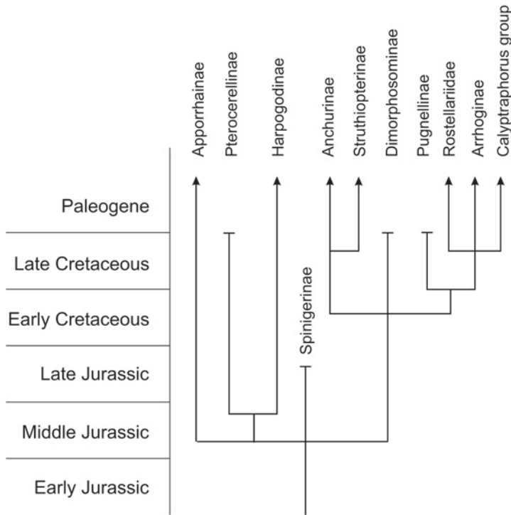
Fig. 7. Relationship between the Mesozoic Aporrhaidae subfamilies and possible origin of the Stromboidae family Rostellariidae and the Calyptrophorus group. Arrows symbolize a distribution beyond the Cretaceous/Paleogene boundary.
