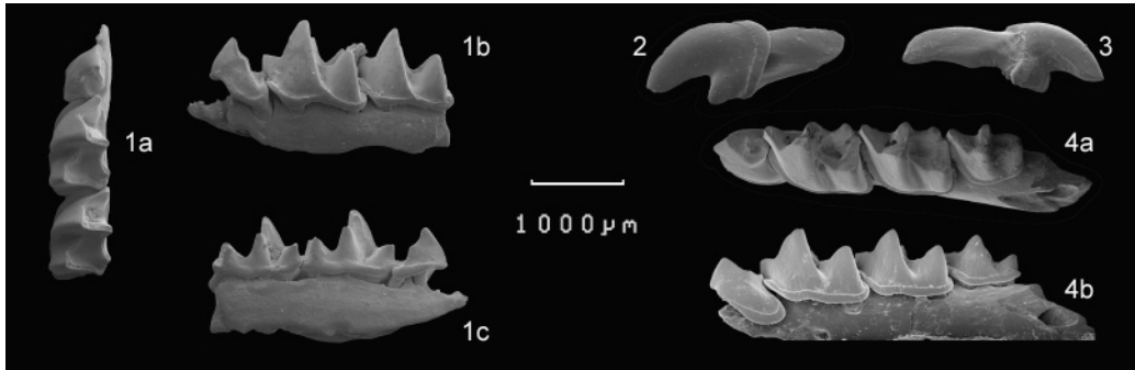
Fig. 25: Crocidurinae gen. et sp. indet. 11 and Sorex sp. ?. 1 : Crocidosoricinae gen. et sp. indet. 11. Right mandibular fragment with p4-m2 (reversed), a. occlusal, b. labial, c. lingual view, Unkheltseg (sample UNCH-A/3, biozone B or D, NHMW 2006z0052/0001); 2.-4 : Sorex sp. ?. 2 : Right I sup. (reversed), labial view, Builstyn Khudag (sample BUK-A/12+14, biozone E, NHMW 2006z0053/0001); 3 : Left I sup., lingual view, Builstyn Khudag (sample BUK-A/12+14, biozone E, NHMW 2006z0053/0002); 4 : Left mandibular fragment with p4-m3, a. occlusal view, b. labial view, Builstyn Khudag (sample BUK-A/12+14, biozone E, NHMW 2006z0053/0003).
