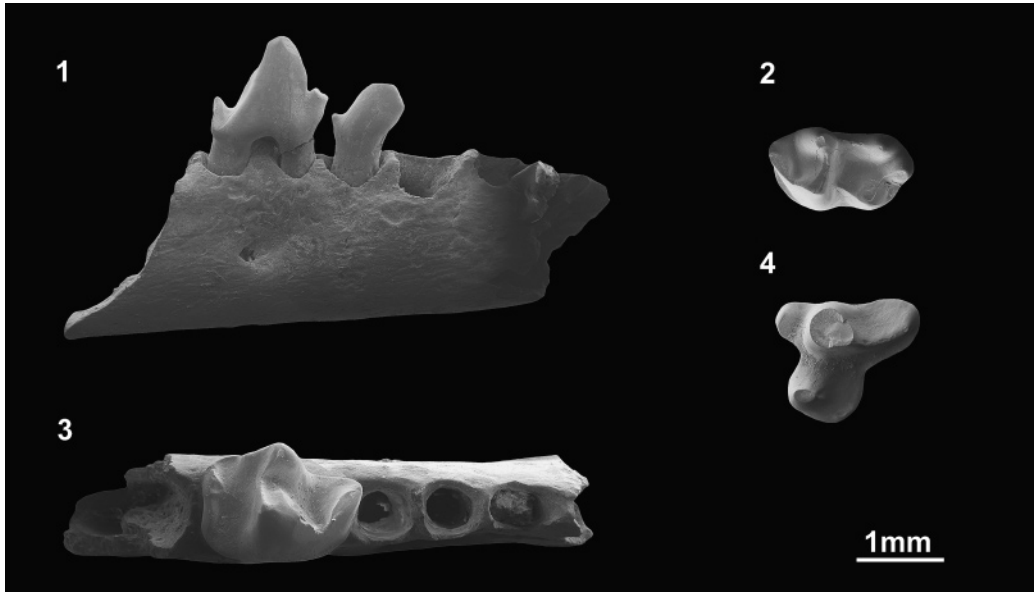
Fig. 5: Zaraalestes sp.: 1 : Right mandibular fragment with p2-p3, labial view, Taatsiin Gol right (sample TGR-AB/21, biozone B, NHMW 2006z0190/0001); 2 : Left m3, occlusal view, Taatsiin Gol right (sample TGR-AB/21, biozone B, NHMW 2006z0190/0003); 3 : Right mandibular fragment with p4, occlusal view, Del (sample DEL-B/7, biozone B, NHMW 2006z0191/0001); 4 : Left P3, occlusal view, Taatsiin Gol right (sample TGR-AB/21, biozone B, NHMW 2006z0190/0002).
