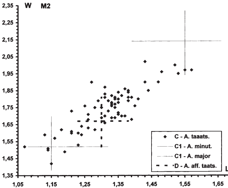
Diagram 2b: Amphelichinus species, scatter diagram of the length and width of M1 and M2.
