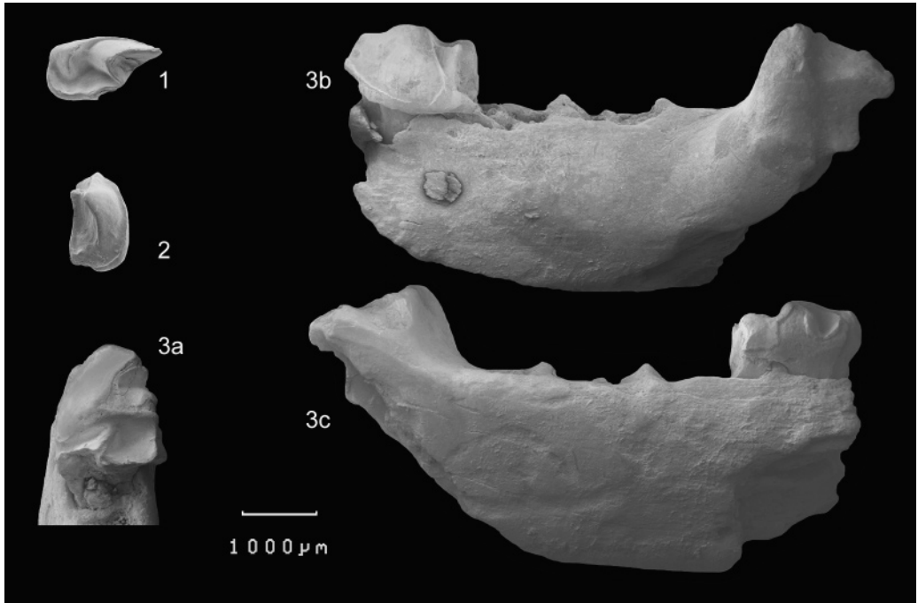
Fig. 18: Heterosoricinae gen. et sp. indet. 1-3: 1 : Heterosoricinae gen et sp. indet. 1. Left M3, occlusal view, Taatsiin Gol Right (sample TGR-AB/21, biozone B, NHMW 2006z0031/0001); 2 : Heterosoricinae gen. et sp. indet. 2. Right A1 (reversed), occlusal view, Hsanda Gol (sample SHG-AB/17-20, biozone B, NHMW 2006z0032/0001); 3 : Heterosoricinae gen. et sp. indet. 3. Left mandibular fragment with m1, a. occlusal view, b. labial view, c. lingual view, Tavan Ovoony Deng (sample RHN-A/7, biozone C1, NHMW 2006z0033/0001).
