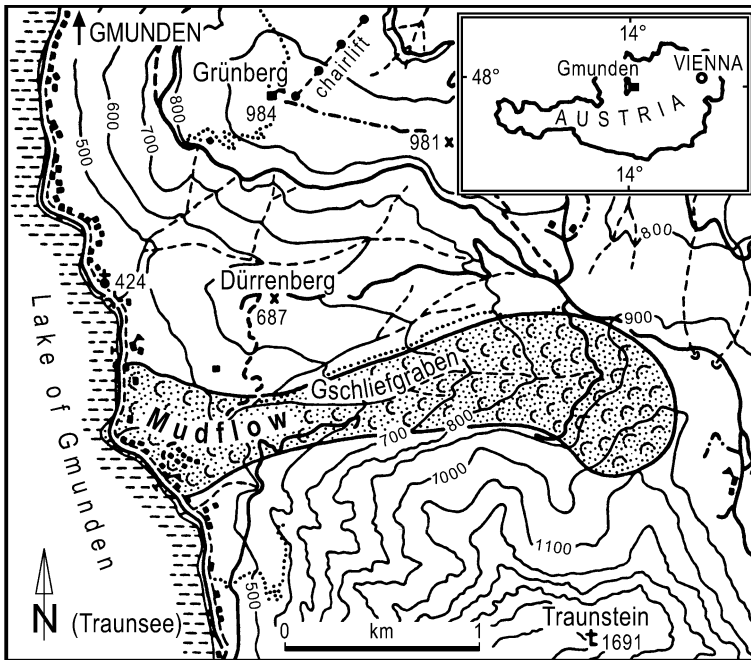
Text-fig. 1: Sketchmap of the Gschliefgraben area (after TRÖGER et al. 1999)
