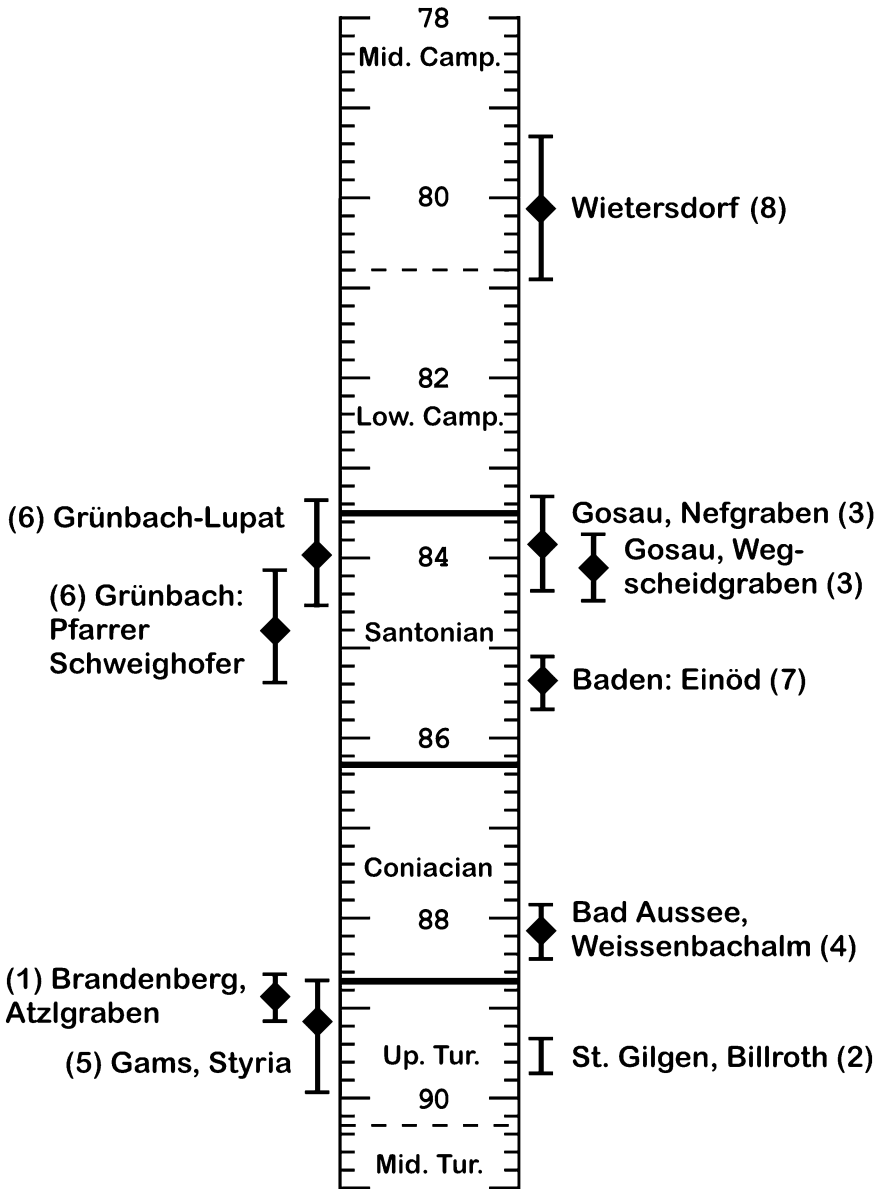
Fig. 2: Numerical ages derived from strontium isotope stratigraphy (Tab. 1) of occurrences of plagiptychids in the Northern Calcareous and Central Alps. Error bars indicate age range due to limits of analytical precision and uncertainty about the seawater Sr-isotope composition (MCARTHUR et al., 2001). Time scale of OBRADOVICH (1993). Numbers given with names of localities refer to those indicated on Figure 1.
