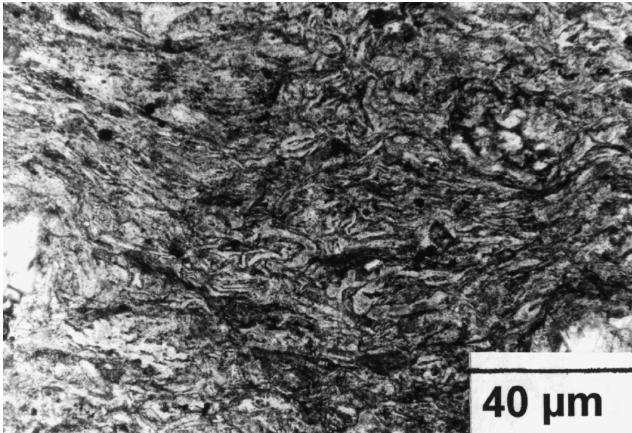
Fig. 10: Optical microscopic image of shard-like relict textures of the welded Gartnerkofel tuff 1. Triassic.
