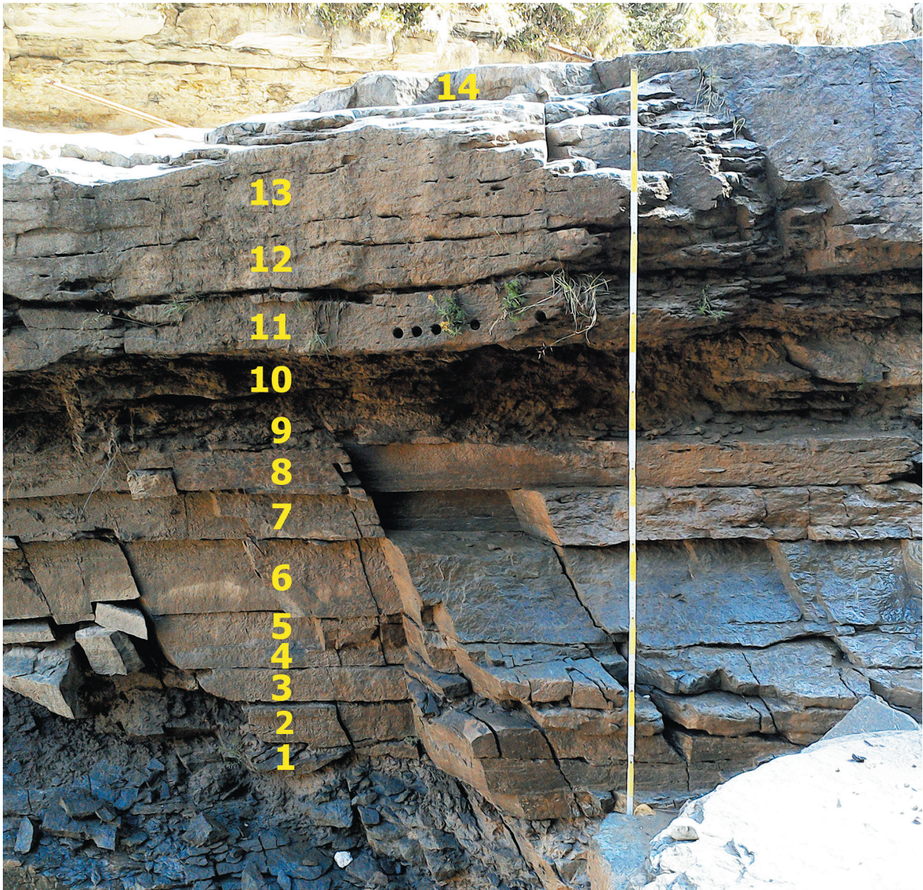
FIG. 5: Skolithos burrows from unit A of the Cephalopod Bank.
