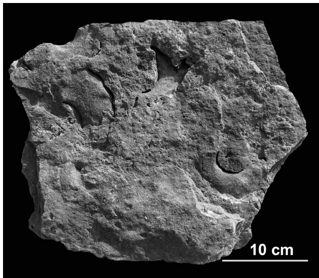
FIG. 7: Slab with "half" nautiloid body chambers, debris, bed 7.
