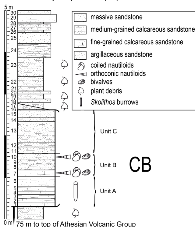
FIG. 3: Stratigraphic column of the Cephalopod Bank at the waterfall outcrop.
