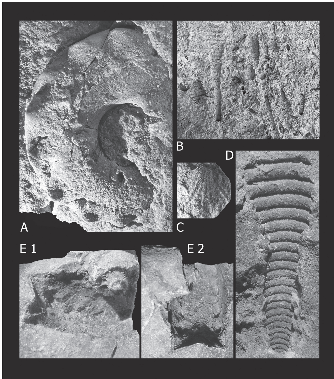
FIG. 6: Coiled and orthoconic nautiloids and pectinoid bivalve from unit B of the Cephalopod Bank. A) internal mold of coiled half-preserved nautiloid from top of bed 7 (x 1); B) parallel oriented orthoconic nautiloids, debris, (x 0.5); C) silicone cast of external mold of pectinoid bivalve, left valve, bed 10, (x 1.5); D) mold of an annulated orthoconic nautiloid, debris, (x 1.5); E1–E2) mold of a vertically embedded coiled nautiloid, E1 lateral view, E2 ventral view, debris (x 1).
